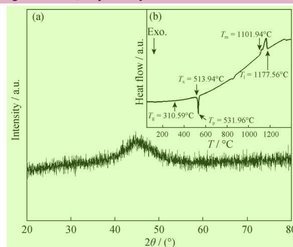
Fig. 1. XRD pattern and DSC curve of the as-milled FeSiBAlNi HEA after 240 h of MA.
