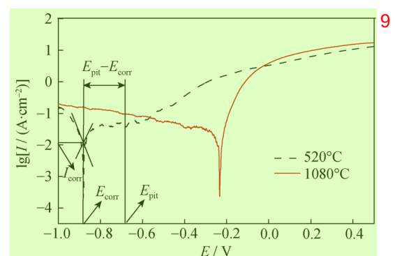
Fig. 5. Potentiodynamic polarization curves of the as-sintered FeSiBAlNi HEA in the seawater solution.
