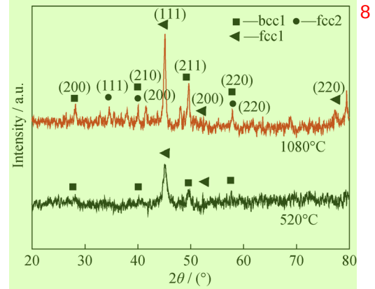
Fig. 2. XRD patterns of the bulk FeSiBAlNi HEA samples sintered at 520 and 1080°C.
